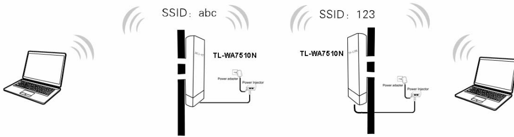
Figure 2-5 Hardware Installation of the TL-WA7510N in Standard AP -- Bridge mode
