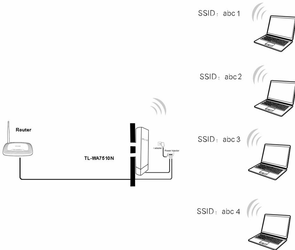
Figure 2-2 Hardware Installation of the TL-WA7510N in Multi-SSID mode
