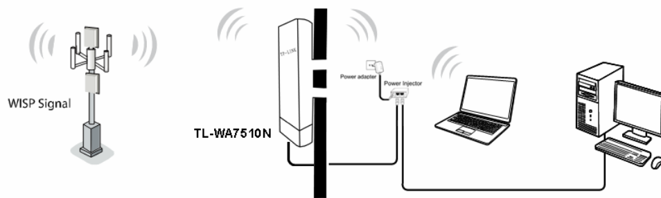
Figure 2-7 Hardware Installation of the TL-WA7510N in AP Client Router mode
