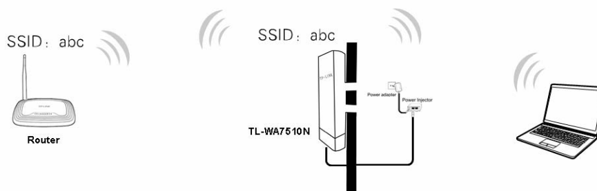
Figure 2-4 Hardware Installation of the TL-WA7510N in (Universal) Repeater mode
