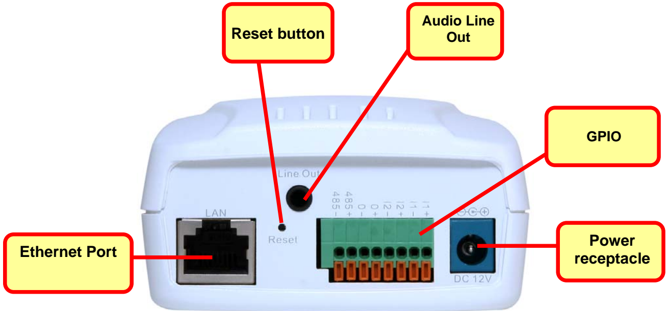
Rear Panel view of TV-IP512P
