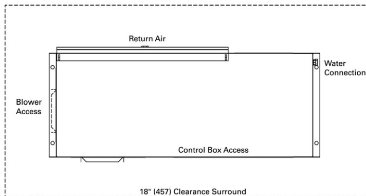
Figure 1: Mechanical clearances - WPHF
