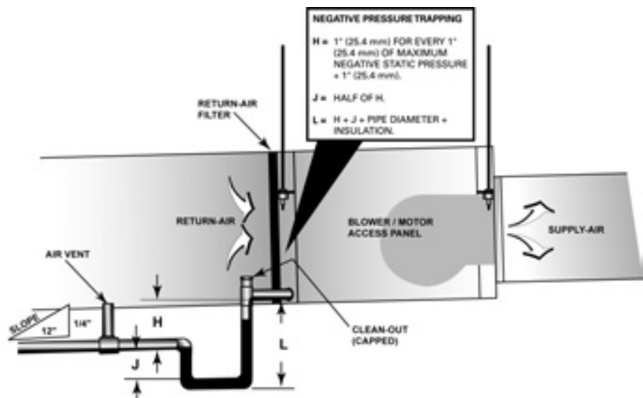
Figure 4: Negative pressure trap
