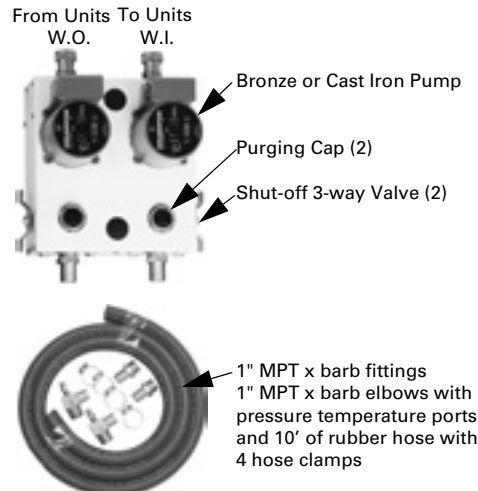
Figure 5: Pump module and hose kit
