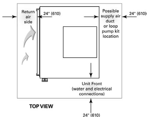
Figure 2: Mechanical clearances - WPVJ
