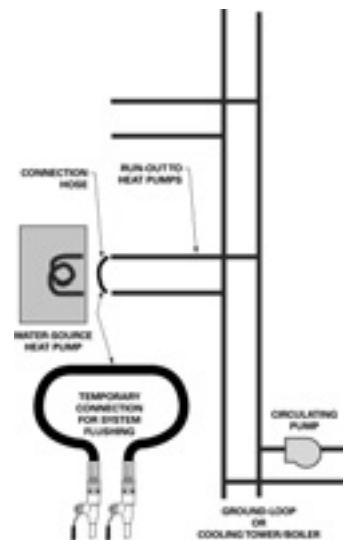
Figure 6: System flushing
