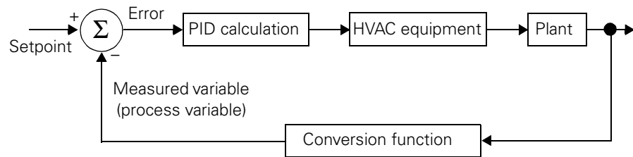
Figure 2: PID loop
