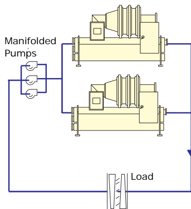
Figure 10. Manifolded pumps
