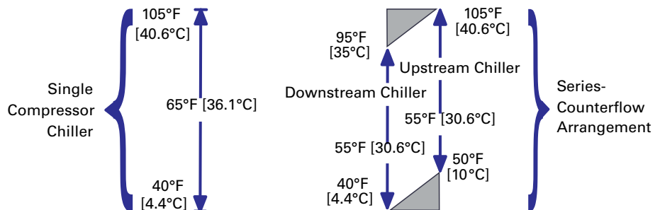
Figure 49. Equal lift concept
