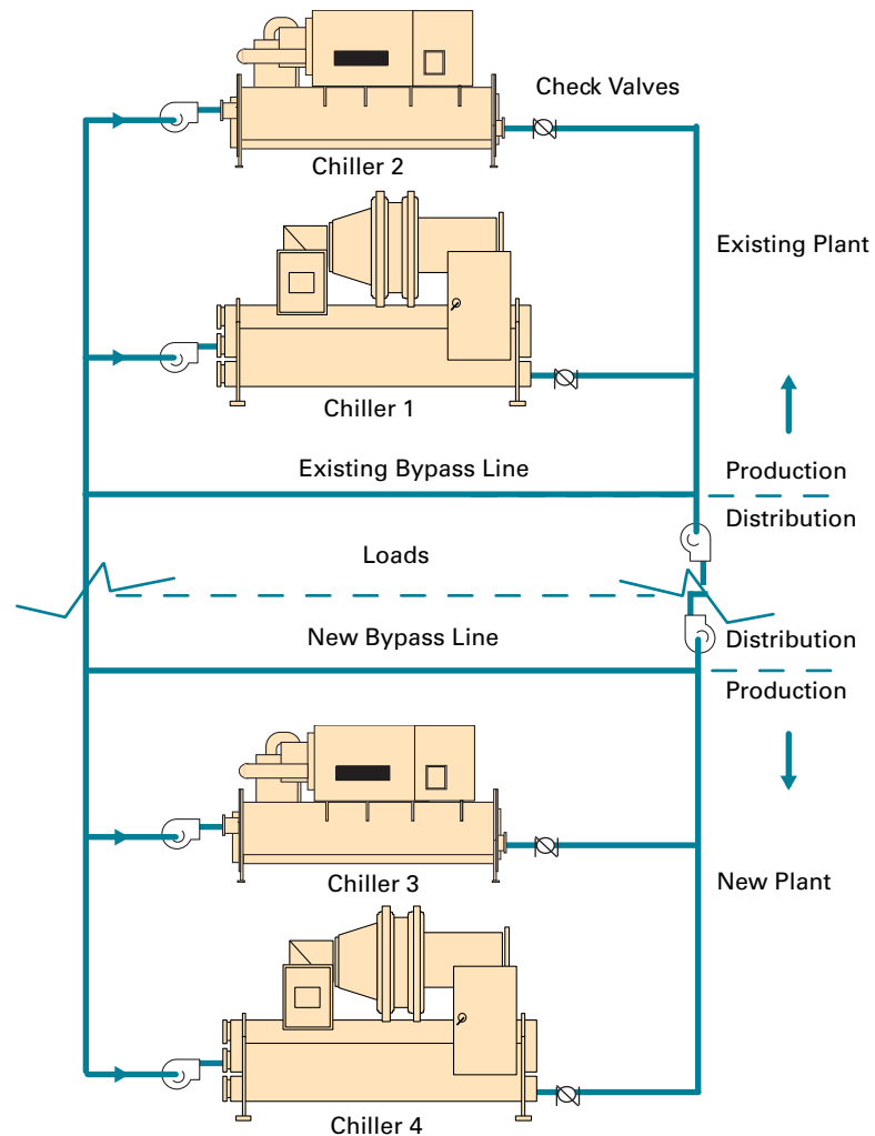
Figure 36. Double-ended decoupled system
