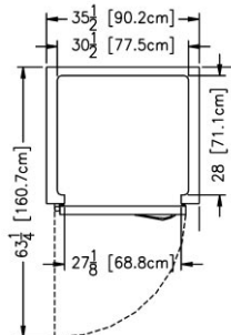
Plan - R/AIF132HUT
