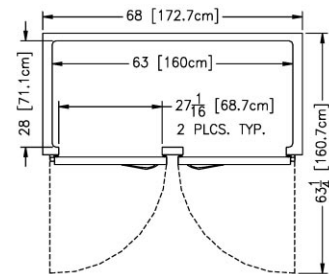
Plan - R/AIF232HUT
