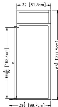
Section - RET232LUT-FHS
