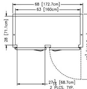
Plan - RET232LUT-FHS
