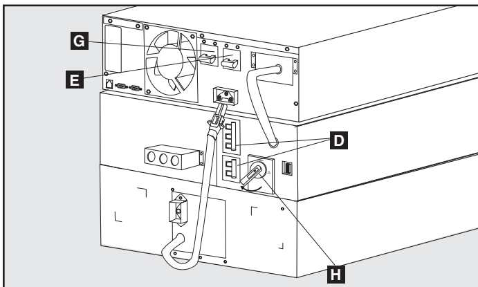
6kVA Models
