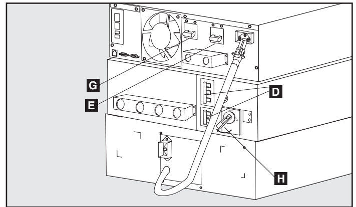
10kVA Models
