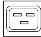
IEC320-C19/230V
