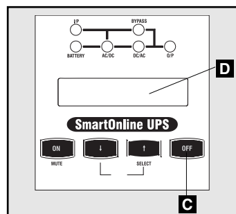
6kVA & 10kVA Models (Front Panel)
