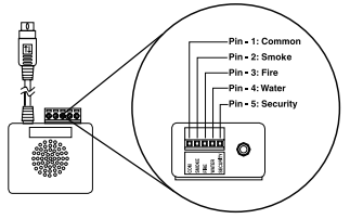
Figure 3: EnviroSense Contact Closure Connections
