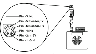
Figure 1: Conector PS/2 EnviroSense
