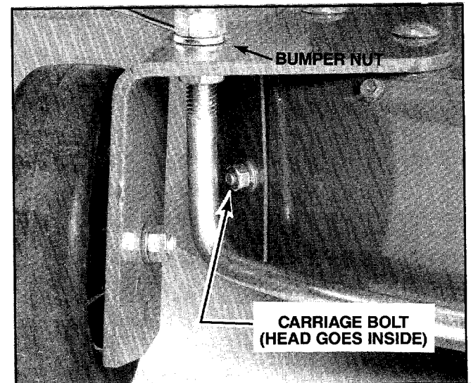
Photo 2-11: Location of fourth carriage bolt.
