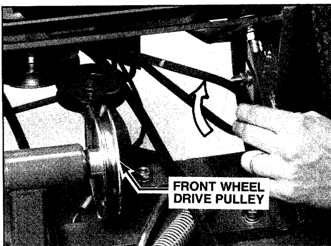
Photo 5-16: Twist belt 1/4 turn clockwise.
