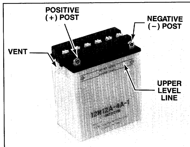
Photo 2-16: Add electrolyte to UPPER LEVEL line.
