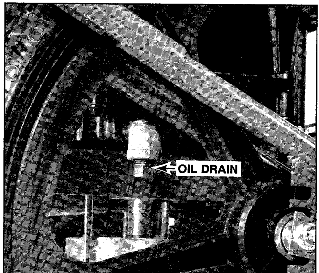
Photo 5-28: Oil drain on 8 HP engine.
