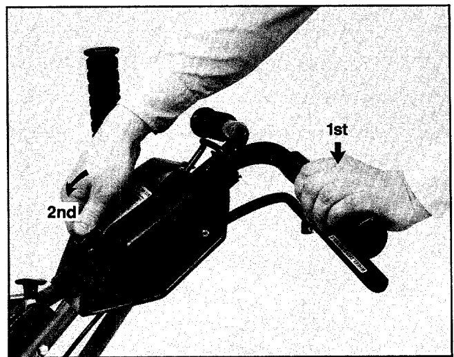
Photo 3-2: Operation of blade control handle and blade control.
