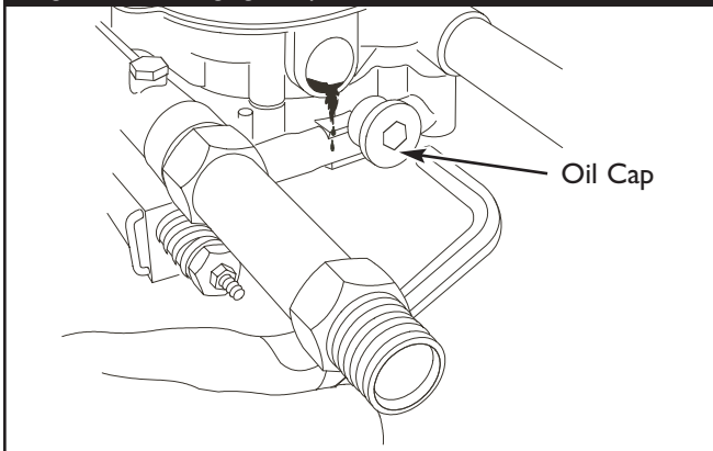
Figure 24 - Changing Pump Oil
