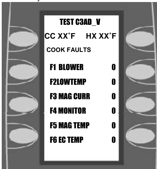
Figure 4-1: Fault
