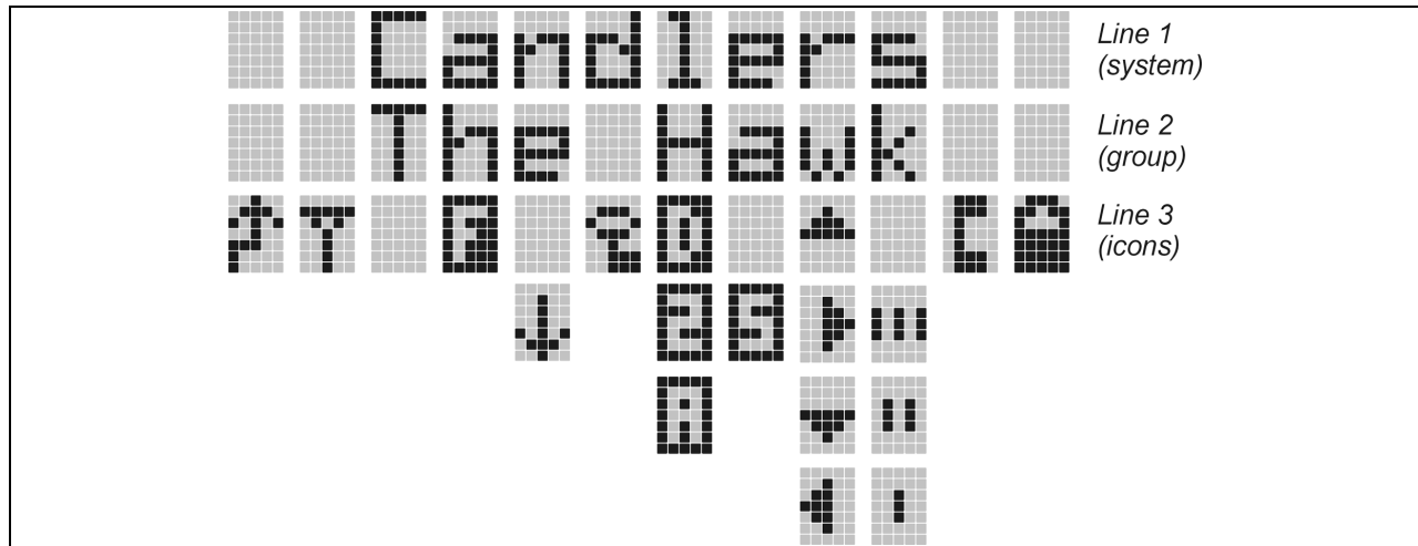
Figure 8-4: Radio Display
