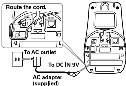
AC adapter
