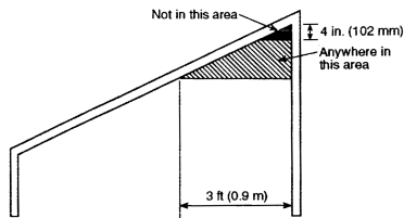
SLOPED CEILINGS (SHED CEILINGS)
