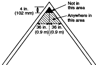
SLOPED CEILINGS (PEAKED CEILINGS)
