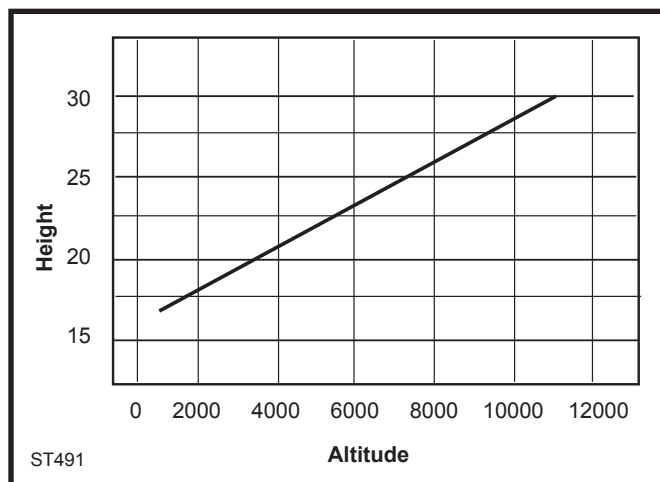
Fig. 2 Chimney height requirements with 152 mm (6") chimney and/or chimney connector.
