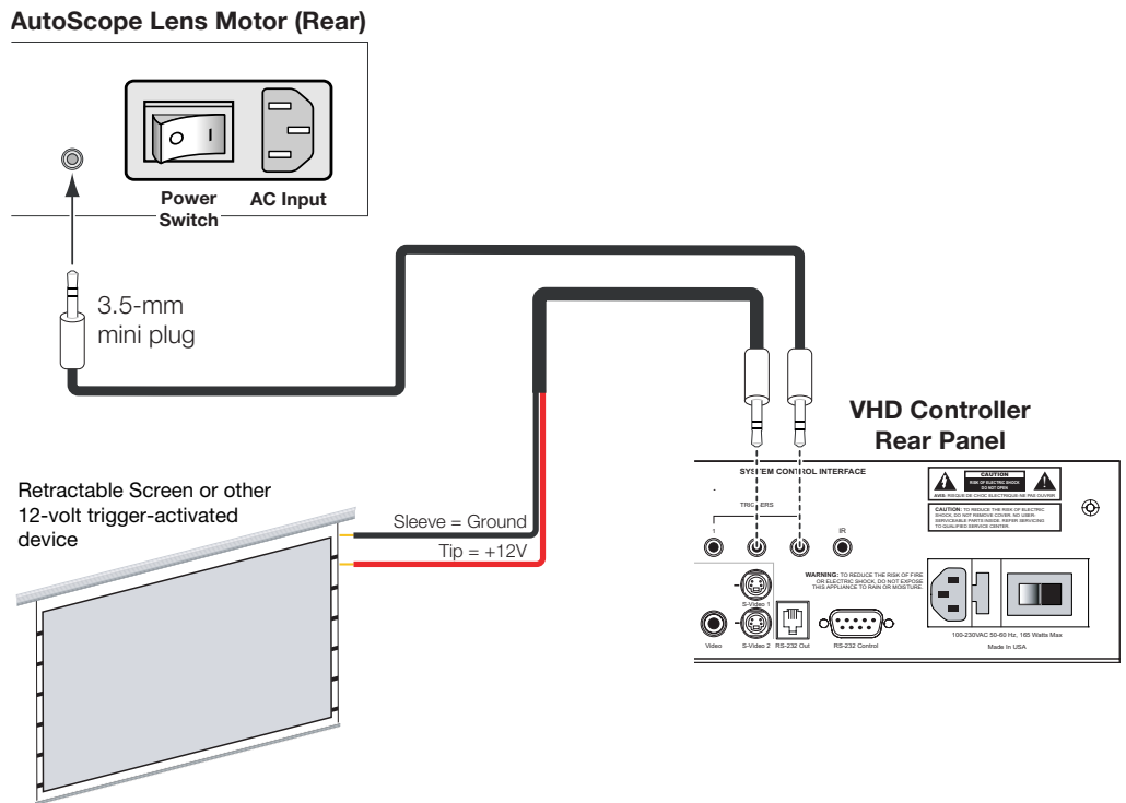
Figure 3-16. 12-volt Trigger Output Connections (from VHD Controller)
