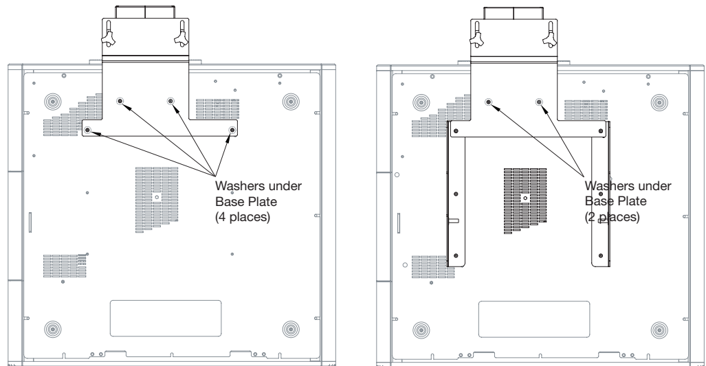
Figure 3-9. Vision 85/CineWide with Anamorphic Lens Base Plate and Ceiling Mounting Rails - Bottom View
