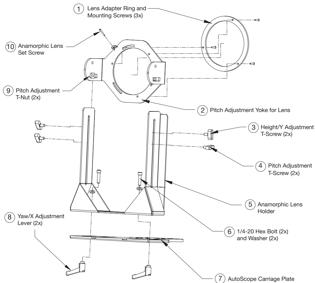
Figure 3-21. Anamorphic Lens Mounting Assembly - Exploded View
