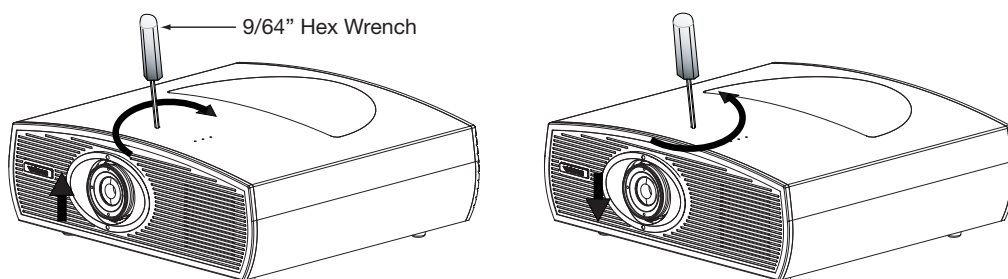
Figure 3-19. Vertical and Horizontal Lens Shift Adjustments
