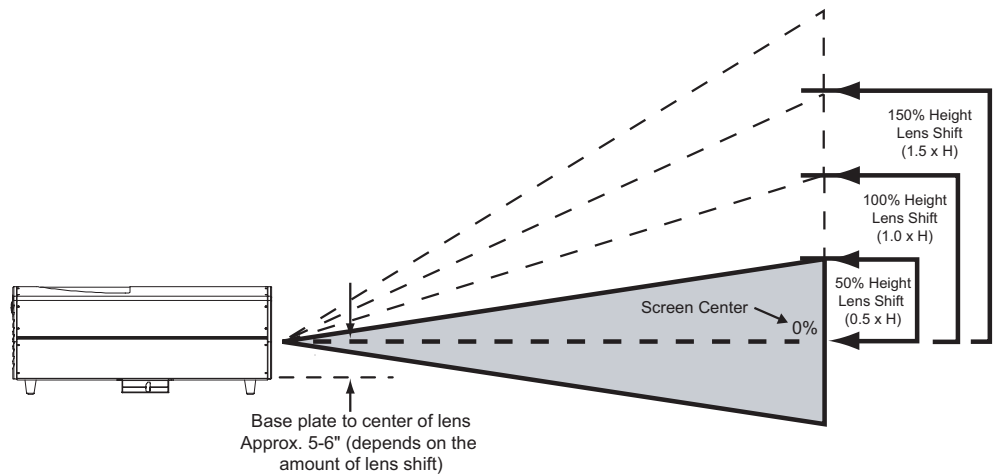
Figure 3-3. Vertical Lens Shift (Example Only)
