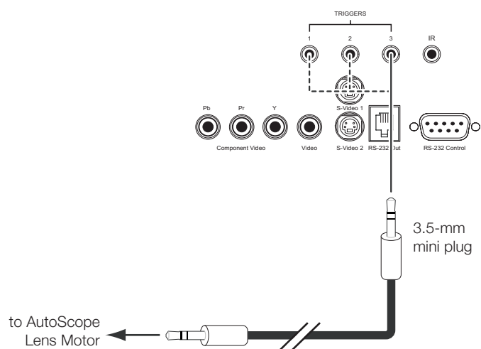
Figure 3-11. Connecting a 12-Volt Trigger Output to the AutoScope Lens Motor
