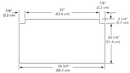
36"W. Cutout w/Downdraft
