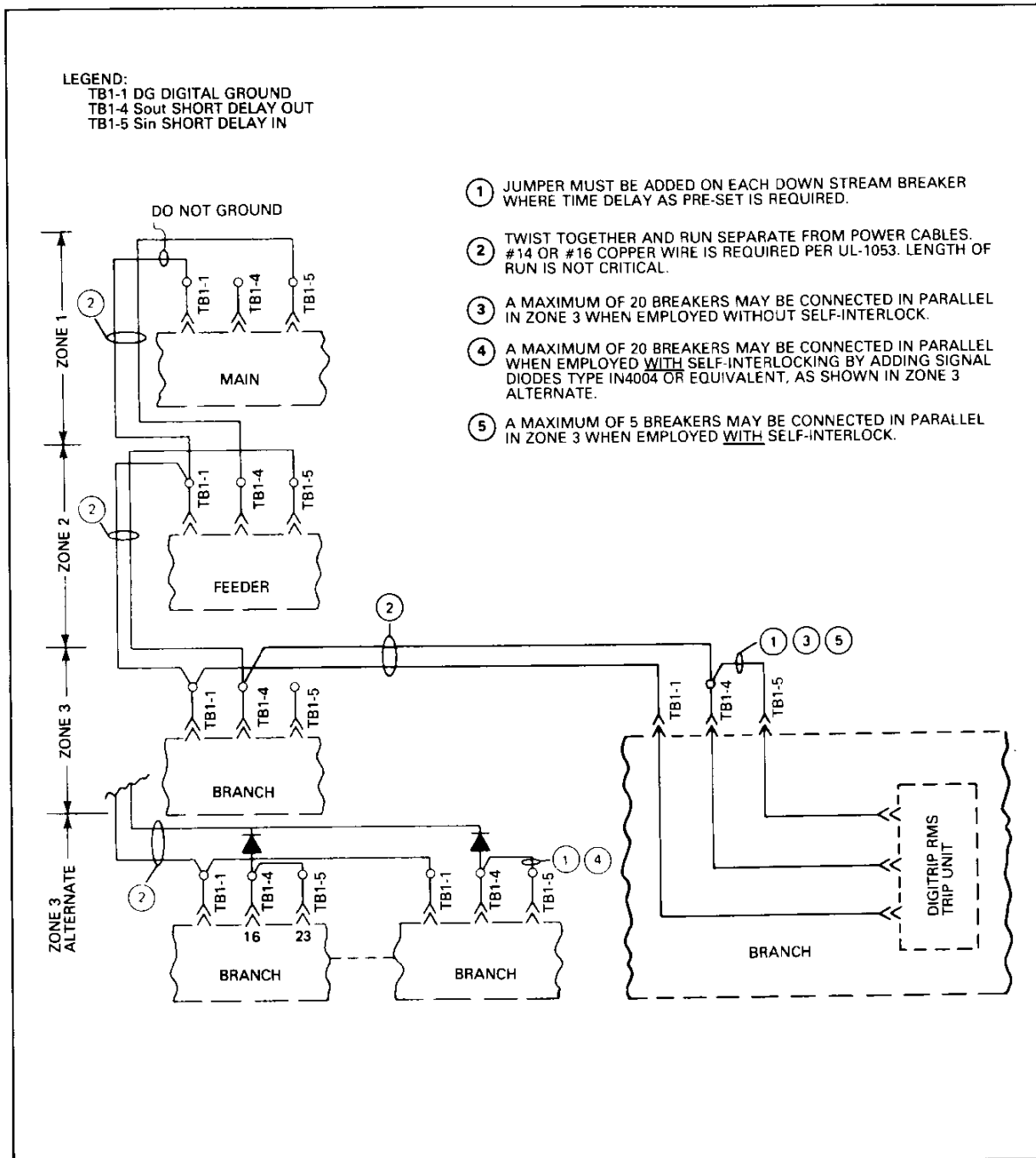
Fig. 13-2. Typical Short Delay Zone Interlocking Connections for Radial Distribution Systems
