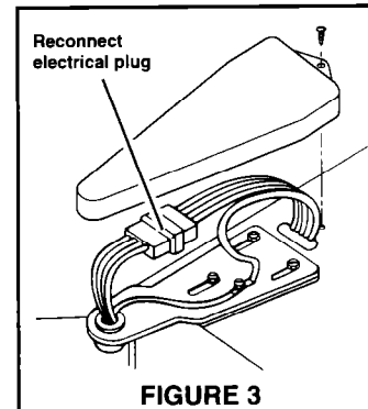
FIGURE 3 FREEZER DOOR ELECTRICAL PLUG
