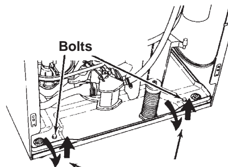
Lift Up On Front of Washer Base
