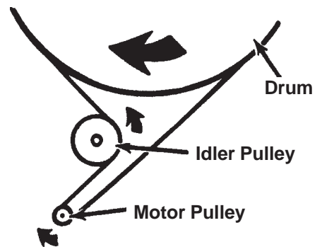
Belt Routing Diagram Viewed From Front
