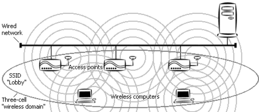
Figure 3. Multiple-AP network
