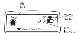
T1-216 Top
