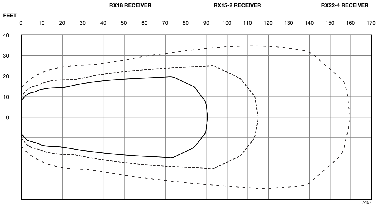
Figure 1: Receiver coverage area with WIR TX75 transmitter OR WIR TX75-S slave emitter in single channel mode.
