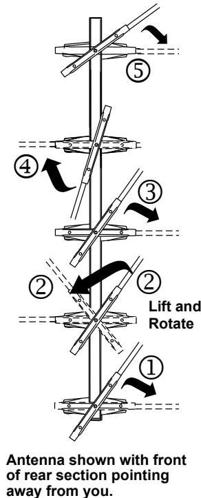
Fig. 1 Model HD7696P
