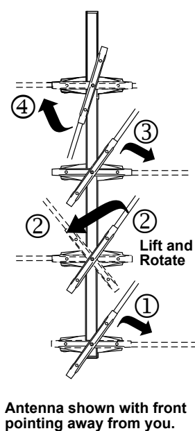
Fig. 1 Model HD7695P
