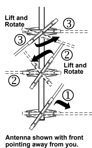
Fig. 1 Model HD7694P
