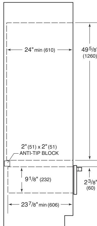
ANTI-TIP BLOCK APPLICATION
