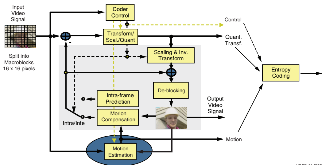
Figure 3-1: H.264 Encoder
