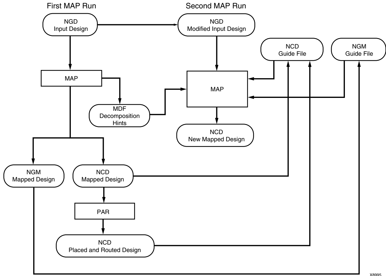
Figure 7-3: Guided Mapping
