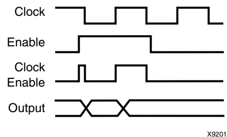
Figure 2-12: Gated Clock
