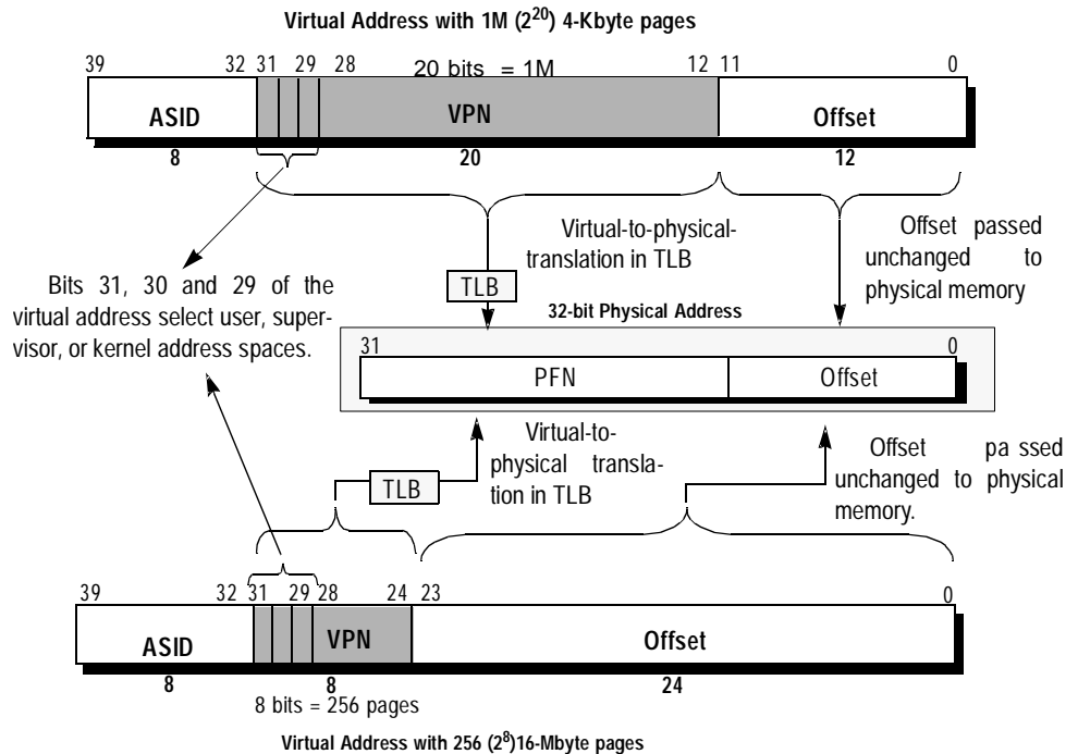
Figure 3: RC32364 Address Translation (Courtesy IDT)
