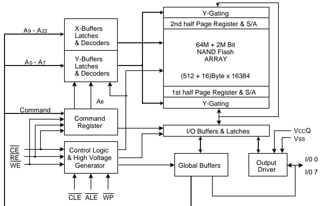
Figure 8: KM29U64000T Block Diagram (Courtesy Samsung Semiconductor)
