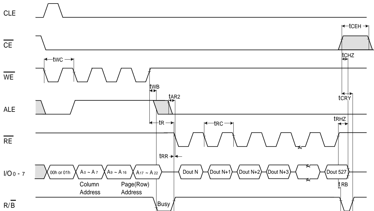
Figure 9: KM29U64000T Read Timing (Courtesy Samsung Semiconductor)
