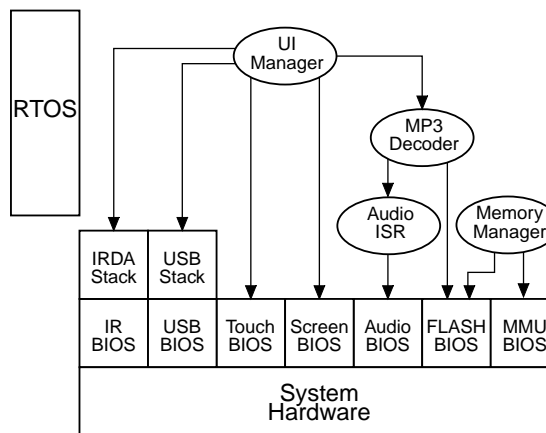
Figure 14: System Software Architecture
