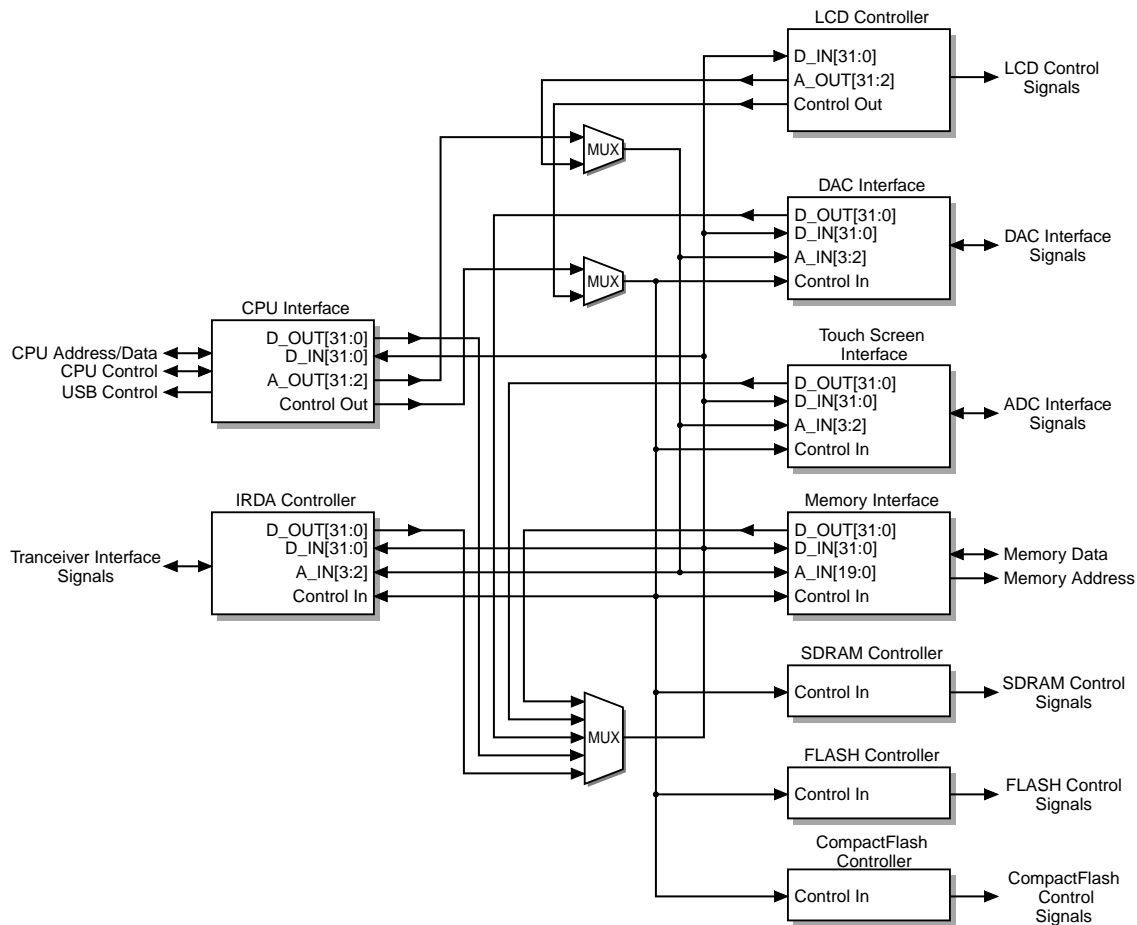
Figure 15: FPGA Logic Block Diagram
