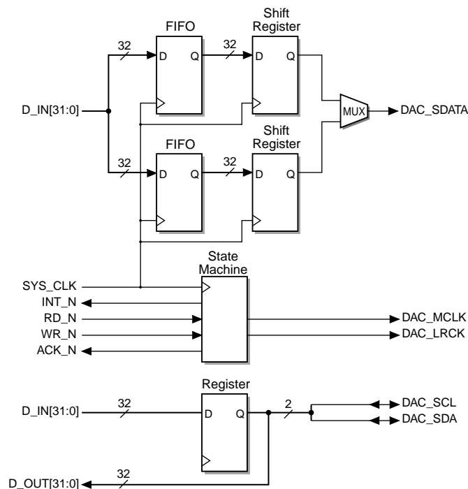
Figure 22: Audio DAC Interface Block Diagram
