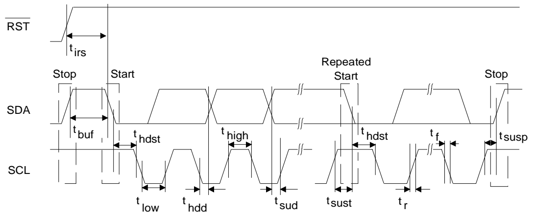
Figure 6: Control Port Timing (Courtesy Cirrus Logic)
