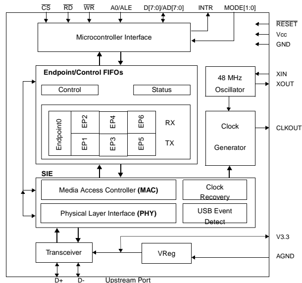
Figure 12: USBN9602 Block Diagram (Courtesy National Semiconductor)
