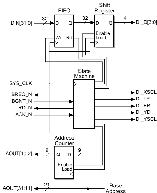
Figure 17: LCD Controller Block Diagram
