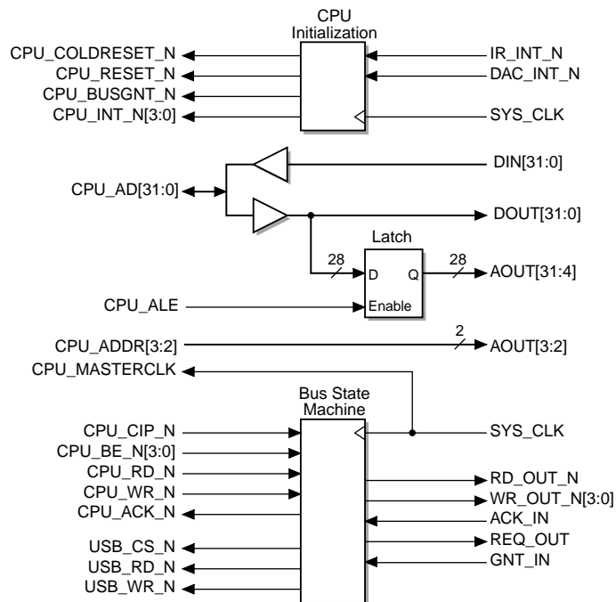
Figure 16: CPU Interface Block Diagram
