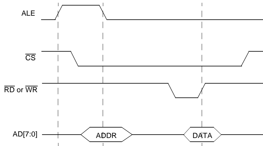
Figure 13: USBN9602 Read / Write Cycle Timing (Courtesy National Semiconductor)
