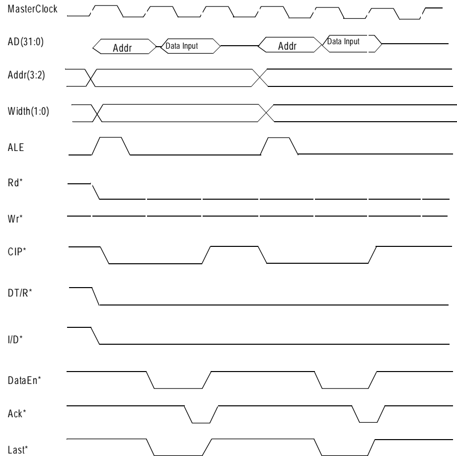
Figure 4: RC32364 Read Timing (Courtesy IDT)
