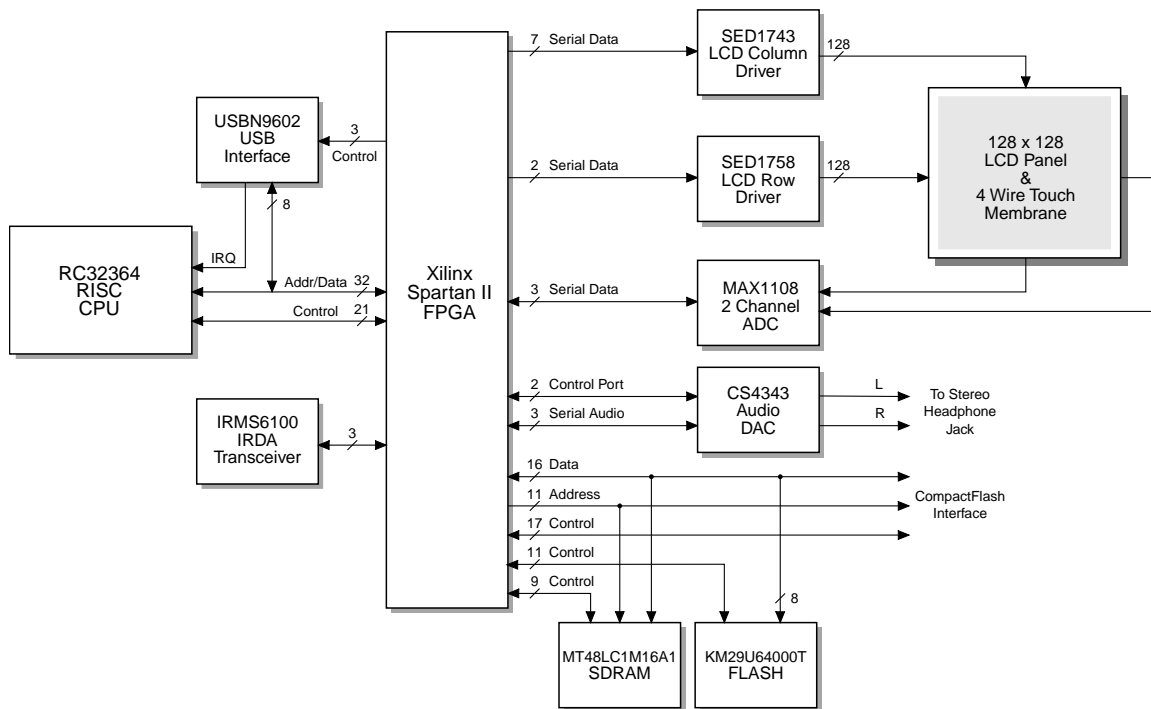
Figure 1: MP3 NG System Block Diagram
