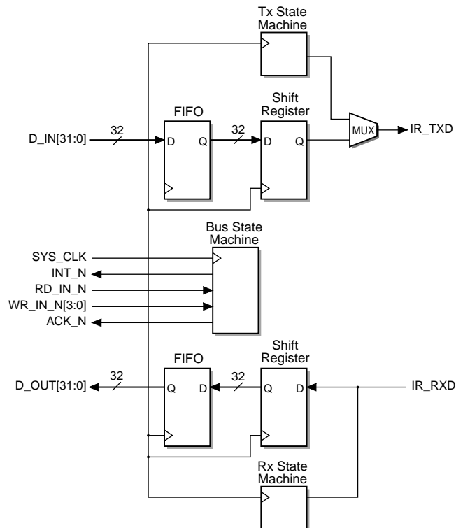
Figure 21: IRDA Controller Block Diagram
