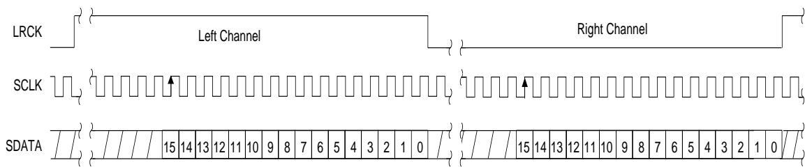
Figure 7: Serial Port Timing (Courtesy Cirrus Logic)
