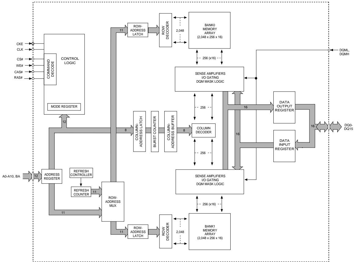
Figure 10: MT48LC1M16A1 Block Diagram (Courtesy of Micron Technology, Inc.)
