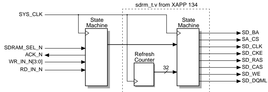
Figure 19: Figure 19 SDRAM Controller Block Diagram
