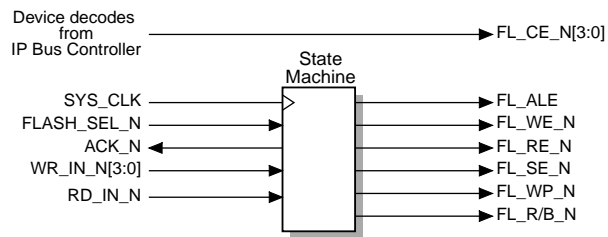
Figure 20: FLASH Controller Block Diagram
