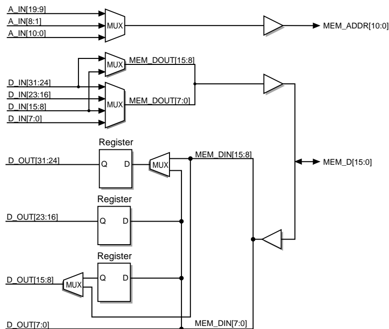
Figure 18: Memory Interface Block Diagram
