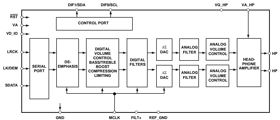
Figure 5: CS4343 Block Diagram (Courtesy Cirrus Logic)
