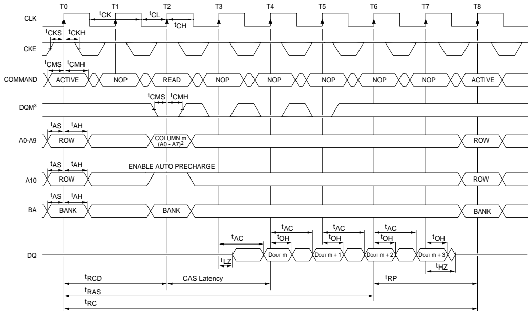
Figure 11: MT48LC1M16A1 Read Timing (Courtesy of Micron Technology, Inc.)
