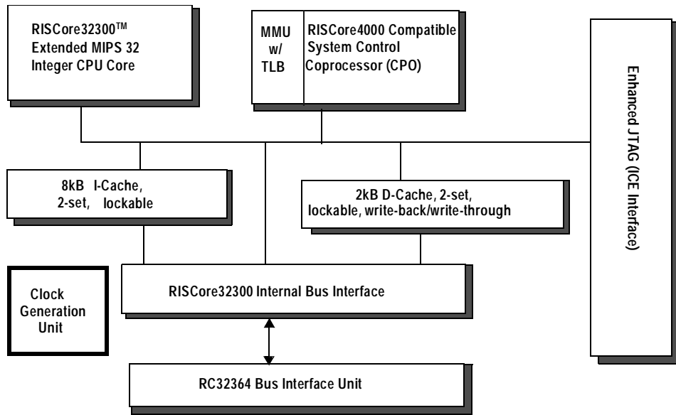
Figure 2: RC32364 Block Diagram (Courtesy IDT)
