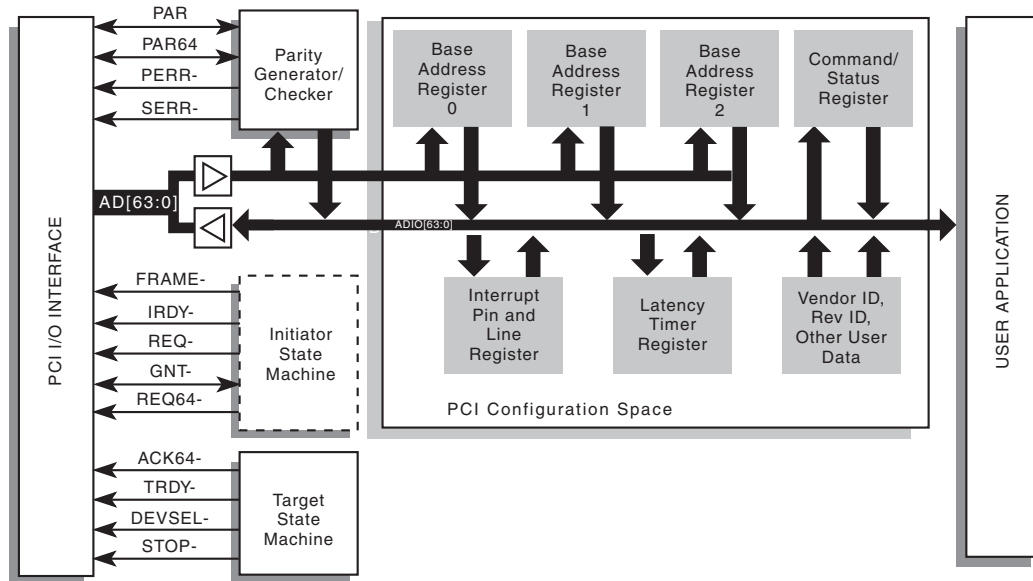
Figure 1: PCI Interface Block Diagram
