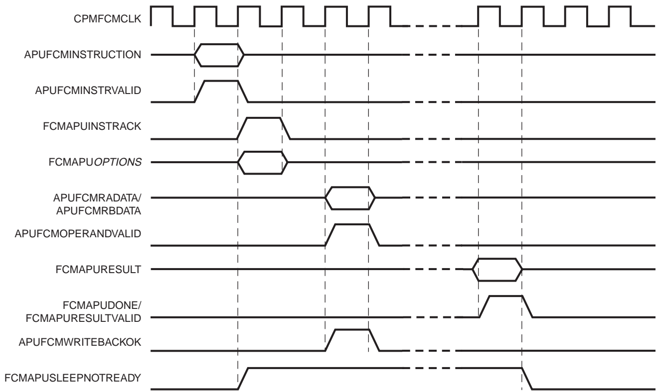
Figure 4-5: FCM Decoded Blocking Transaction Example
