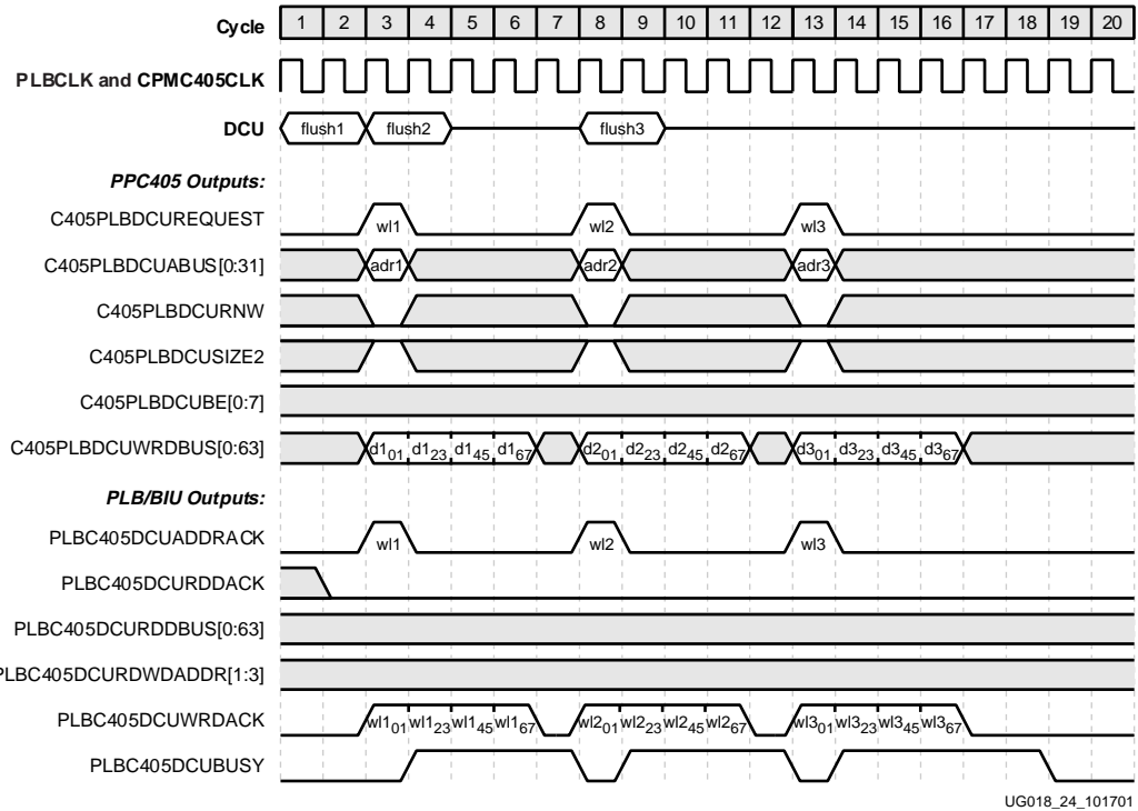
Figure 2-20: DSPLB Three Consecutive Line Writes
