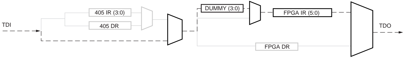
Figure 2-39: Default Instruction Register Data Path in Virtex with Single PPC405 core
