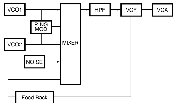
Block Diagram
