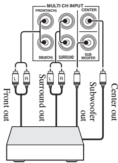
Multi-format player/External decoder (5.1-channel output)
