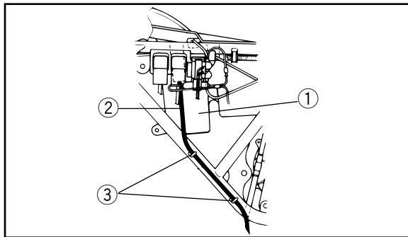
1. Battery 2. Battery breather hose 3. Guide (x 2)
