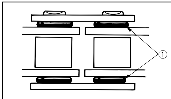
1. O-rings
