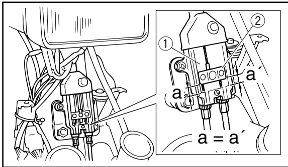
1. Equalizer
