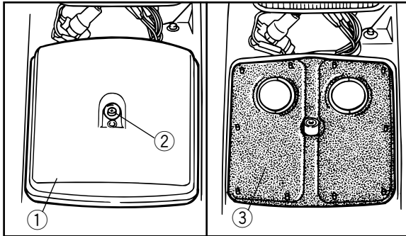
1. Element cover 2. Screw 3. Element
