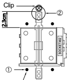
Heat sink attach holes
