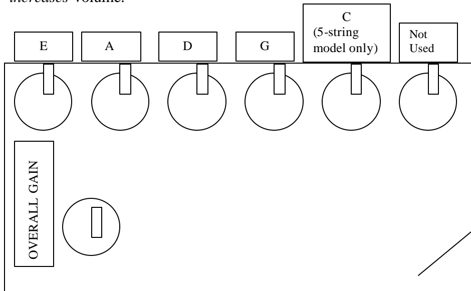
Diagram - Internal Preamp and Trim Pot Controls
