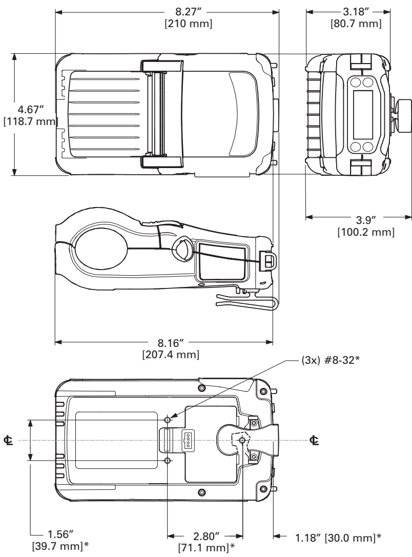
Figure 28: QL 320 Overall Dimensions
