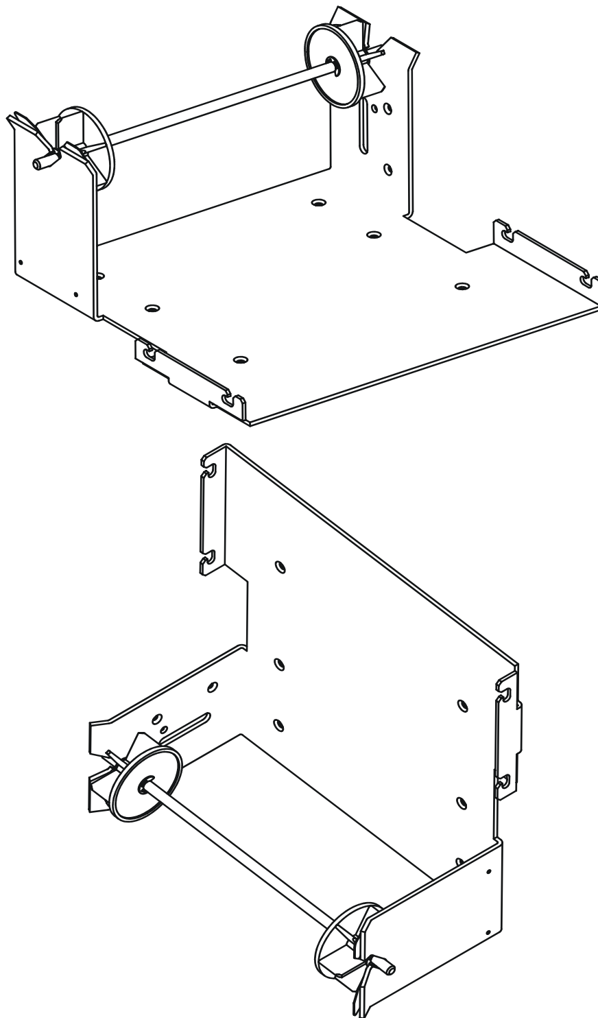
Figure 26 • Combo Roll Holder 01861-21x for Standard, Compact, and Vertical Versions of the Printer
