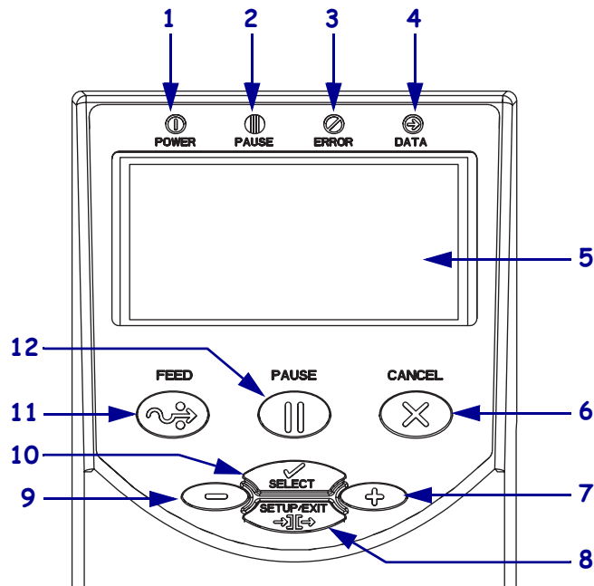
Figure 5 • Control Panel
