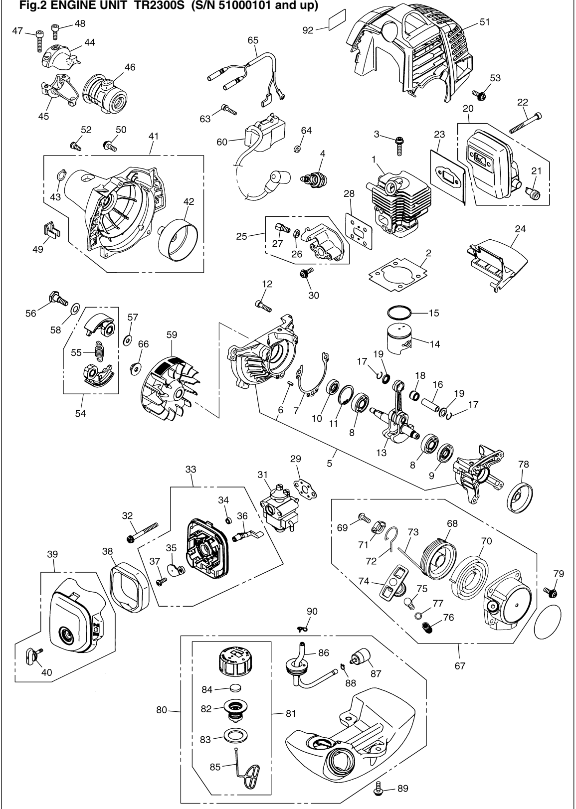
Fig.2 ENGINE UNIT TR2300S (S/N 51000101 and up)
