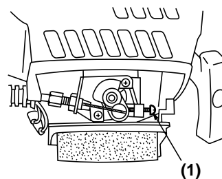
(1) Idle adjusting screw
