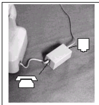
Figure 1-1. Desk Mount Filter Connections
