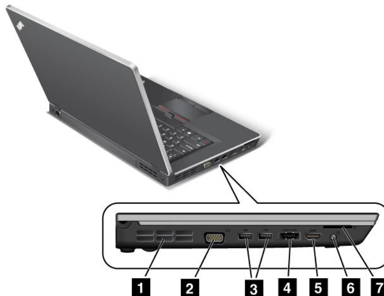
Figure 4. ThinkPad Edge E420 and E520 left-side view
