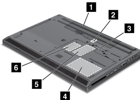
Figure 4. ThinkPad L430 and L530 bottom view
