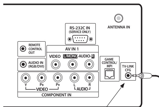
TV-LINK CFG Use for direct PC-to-TV FTG configuration.
