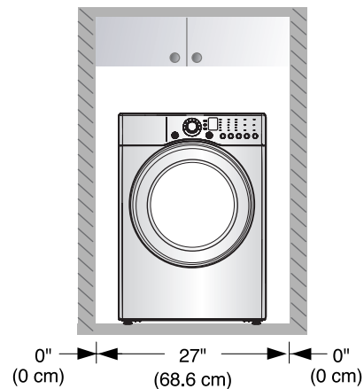
Closet-front View
