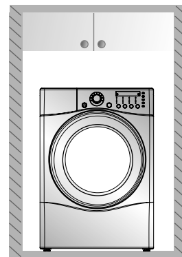
1" (2.54 cm) 27" (68.6 cm) 1" (2.54 cm)
